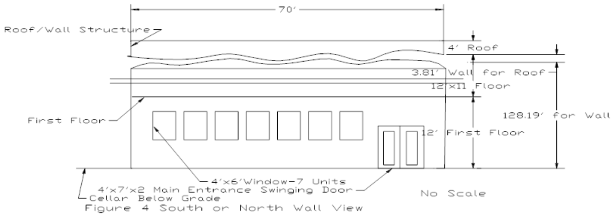
Figure A1. Building vertical plan.
