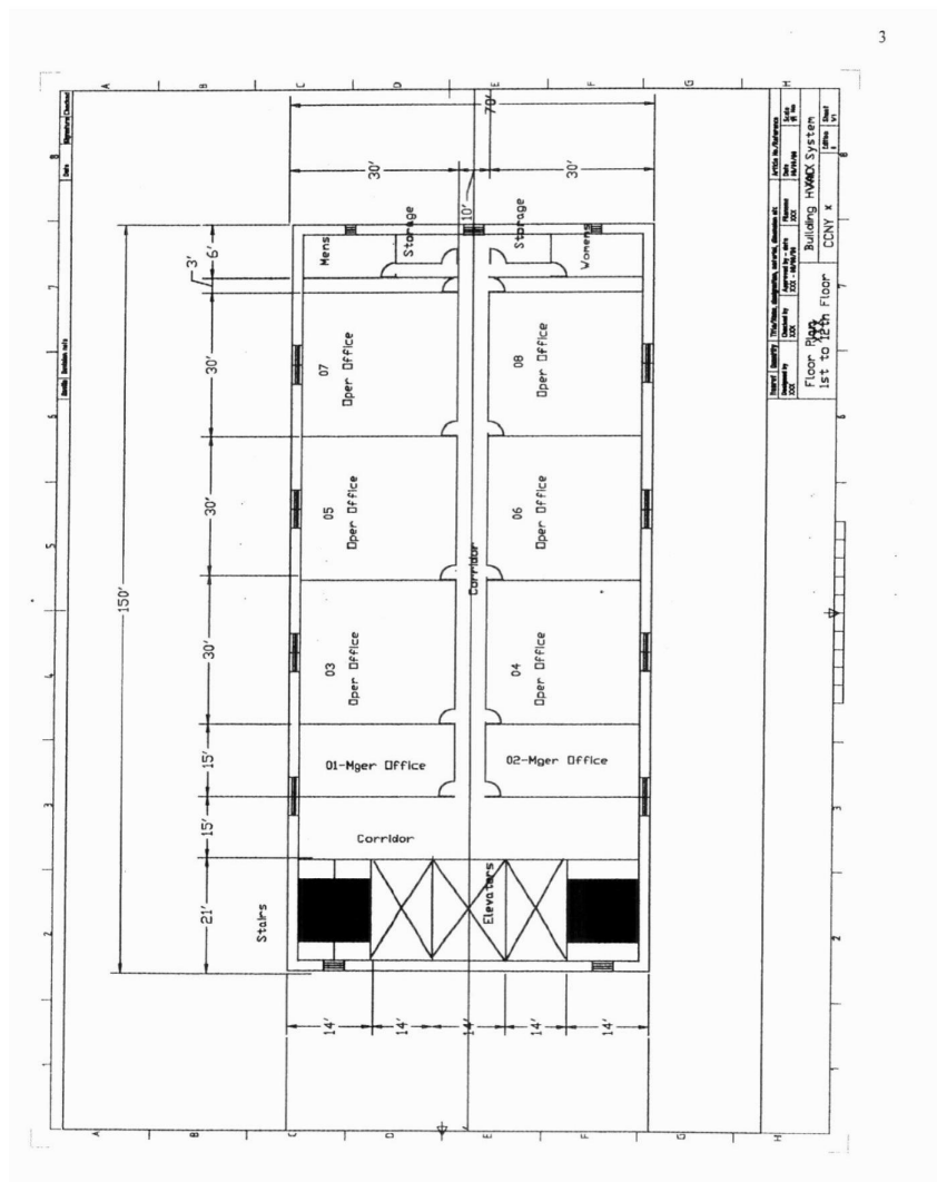
Figure A2. Building floor plan layout.
