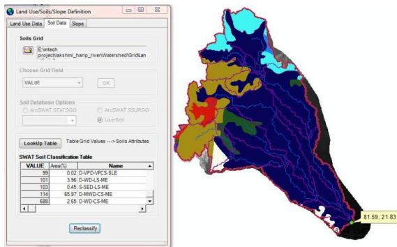
Figure 11. Comparison of Peak Runoff Events across Different Watersheds.
