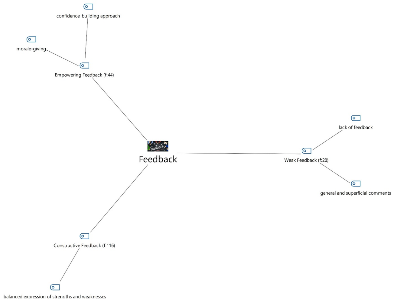
Figure 4. Feedback Practices.
