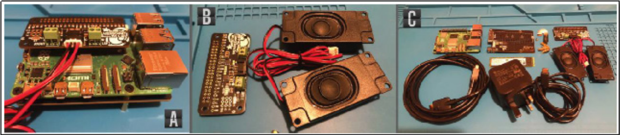
Figure 6. The Raspberry Pi 5 platform with the Adafruit Stereo Bonnet on top (A); the Adafruit Bonnet with the 3W Speakers (B); all the Raspberry Pi 5 attachable components (C)
