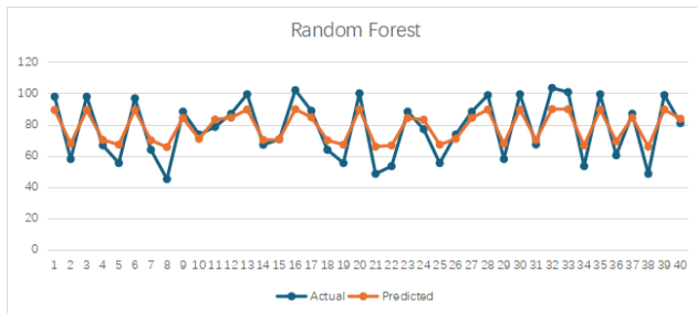
Figure 5. Random Forest.
