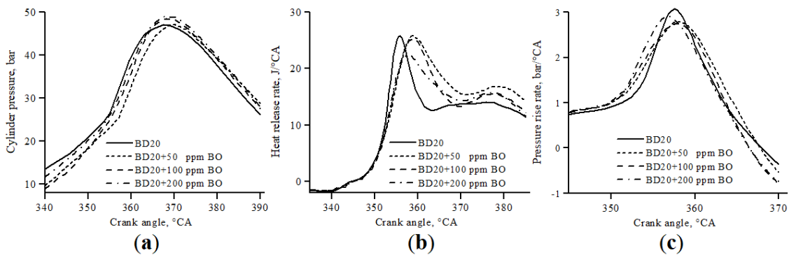
Figure 10. Variation of (a) cylinder pressure; (b) heat release rate; and (c) pressure rise rate with addition of BO to diesel-biodiesel (BD20) blend [31].
