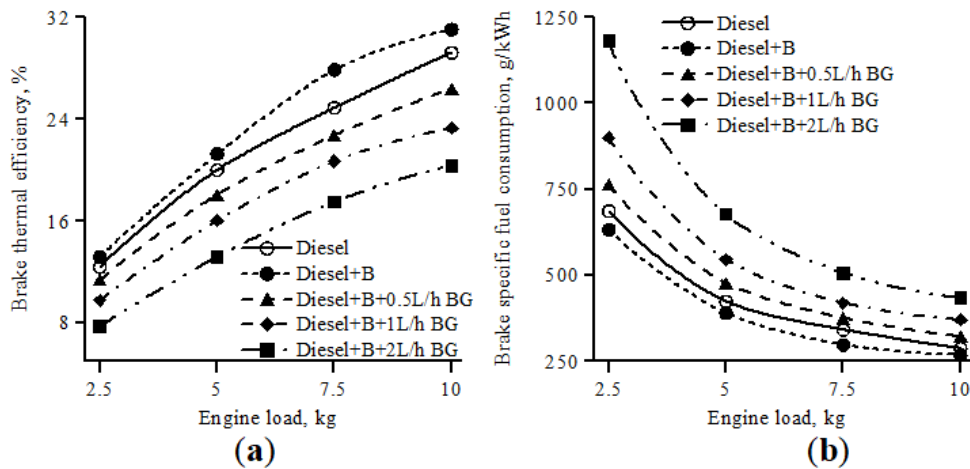
Figure 33. Variation of (a) brake thermal efficiency; and (b) brake specific fuel consumption with engine load for different amount of boron (B) nanoparticles addition to diesel-biogas (BG) dual fuel engine [33].
