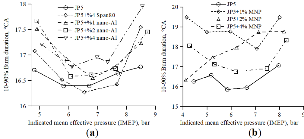
Figure 19. Variation of burn duration for addition of (a) n-Al nanoparticles; and (b) Ti-Al-B metallic nanoparticles (MNP) mixture to JP5 fuel [34].
