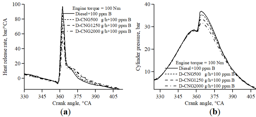
Figure 13. Variation of (a) heat release rate; and (b) cylinder pressure for diesel–CNG dual fuel engine during 100 ppm B addition [32].
