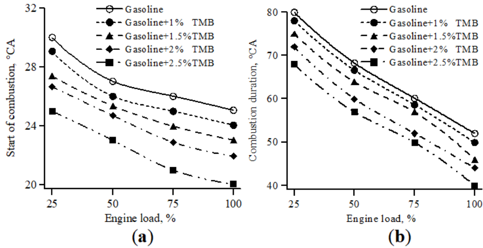
Figure 5. Variation of (a) start of combustion; and (b) combustion duration for addition of TMB to gasoline [19].
