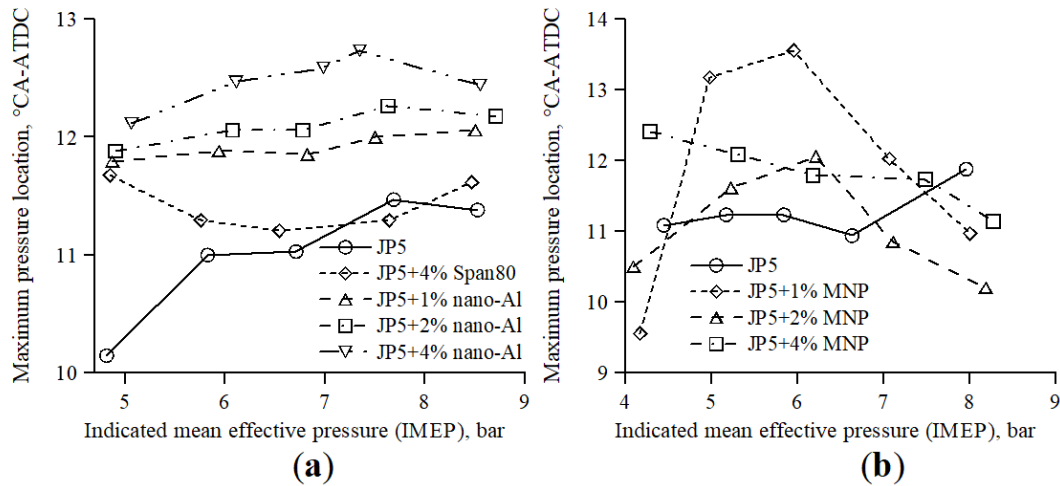
Figure 17. Variation of maximum pressure location for addition of (a) n-Al nanoparticles; and (b) Ti-Al-B metallic nanoparticles (MNP) mixture to JP5 fuel [34].
