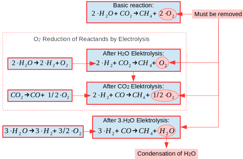
Figure 6. Process Description of the Thermal Methanation.
