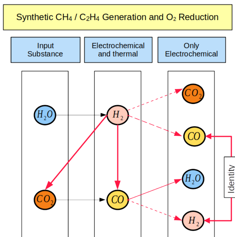
Figure 5. Structural Investigation of Possible Reversible Process Combinations.
